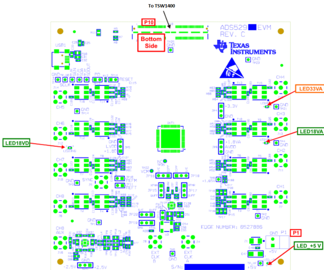
Figure 4. Power-Up Indications
