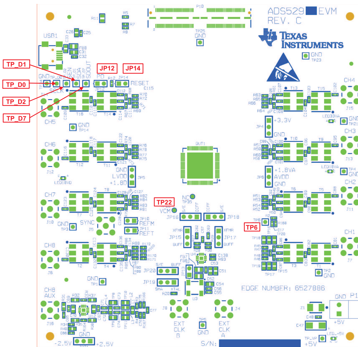
Figure 14. ADS5292EVM Test Point Locations
