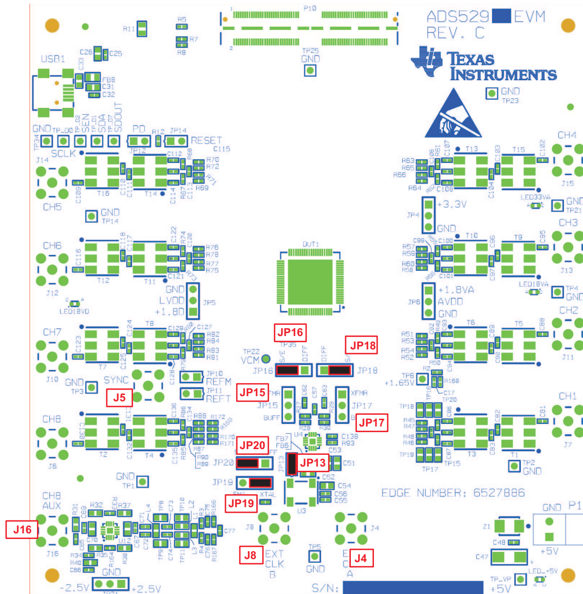
Figure 12. ADS5292EVM Default Clock Jumper Locations
