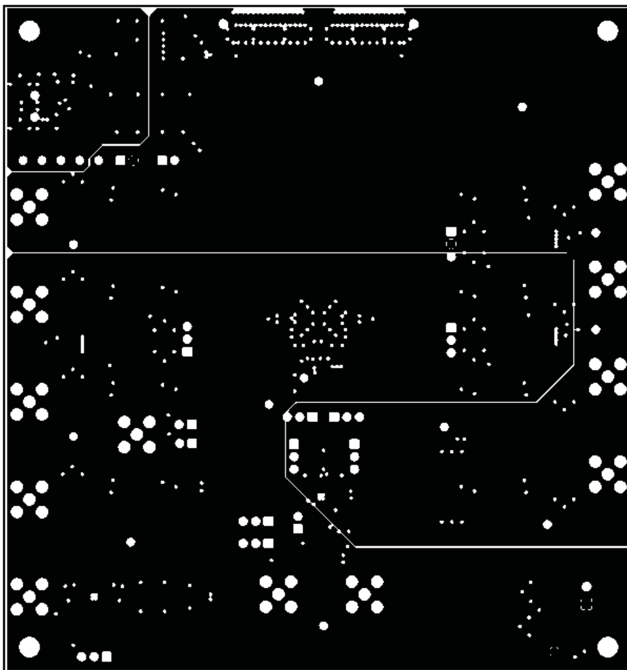
Figure 28. ADS5292EVM Internal Layer 2, Power – Top View
