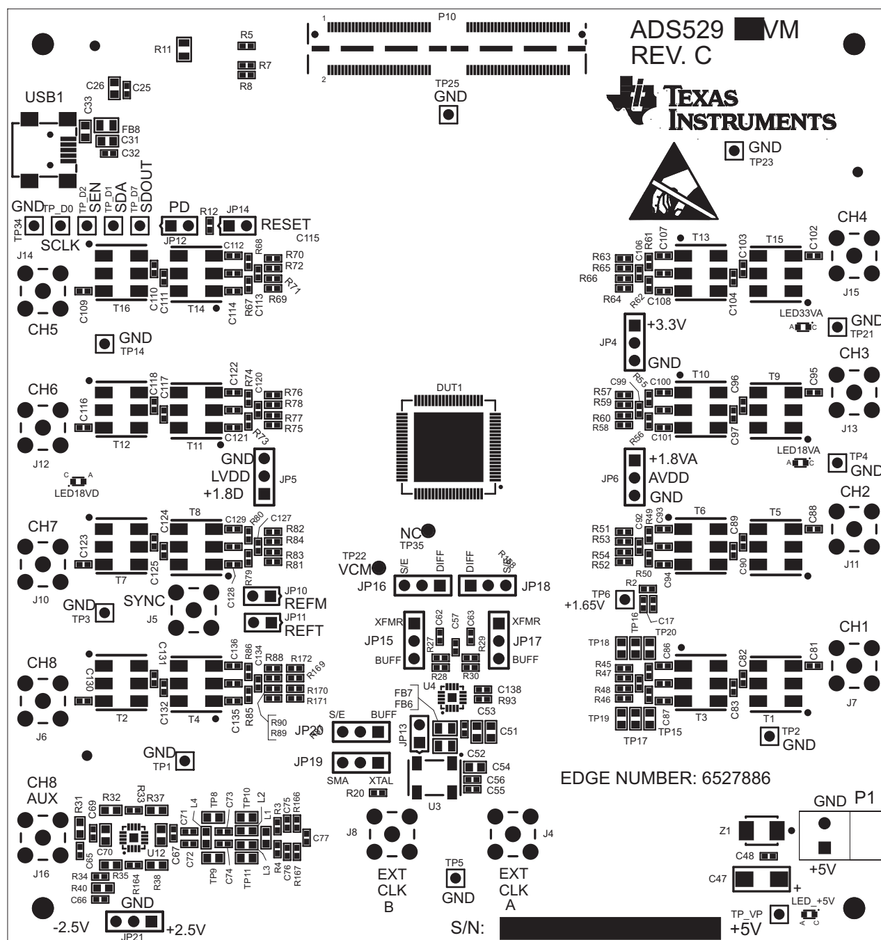
Figure 24. ADS5292EVM Top Layer Assembly Drawing – Top View
