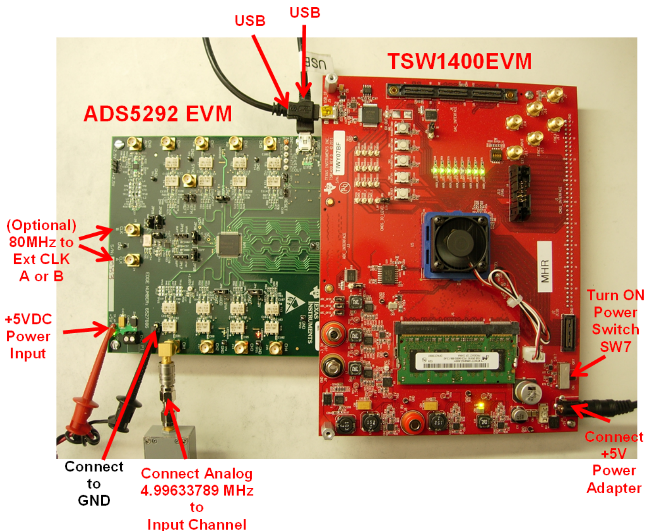
Figure 3. HW Setup With Connection Between TSW1400EVM and ADS5292EVM
