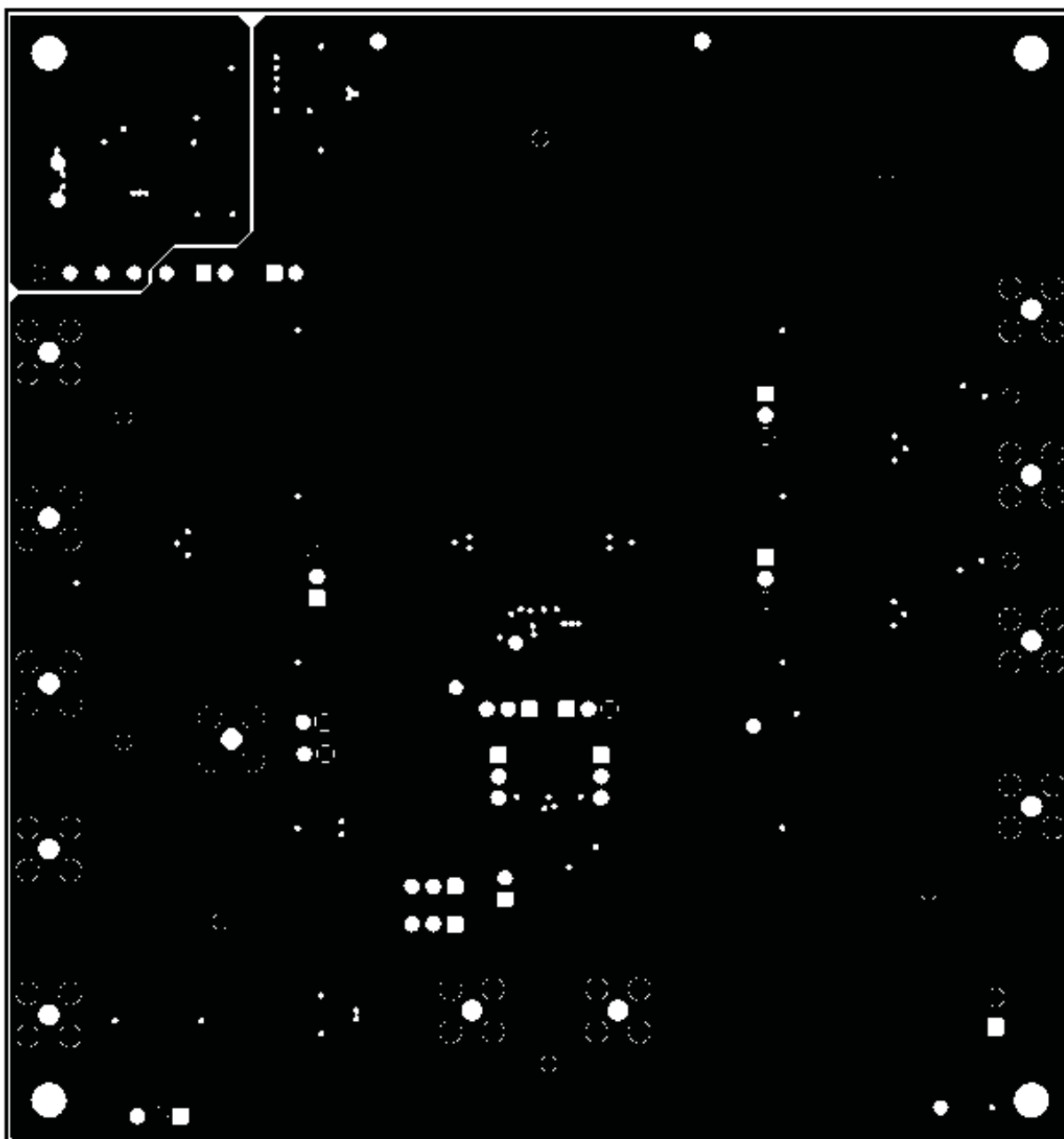
Figure 30. ADS5292EVM Internal Layer 4, Ground – Top View
