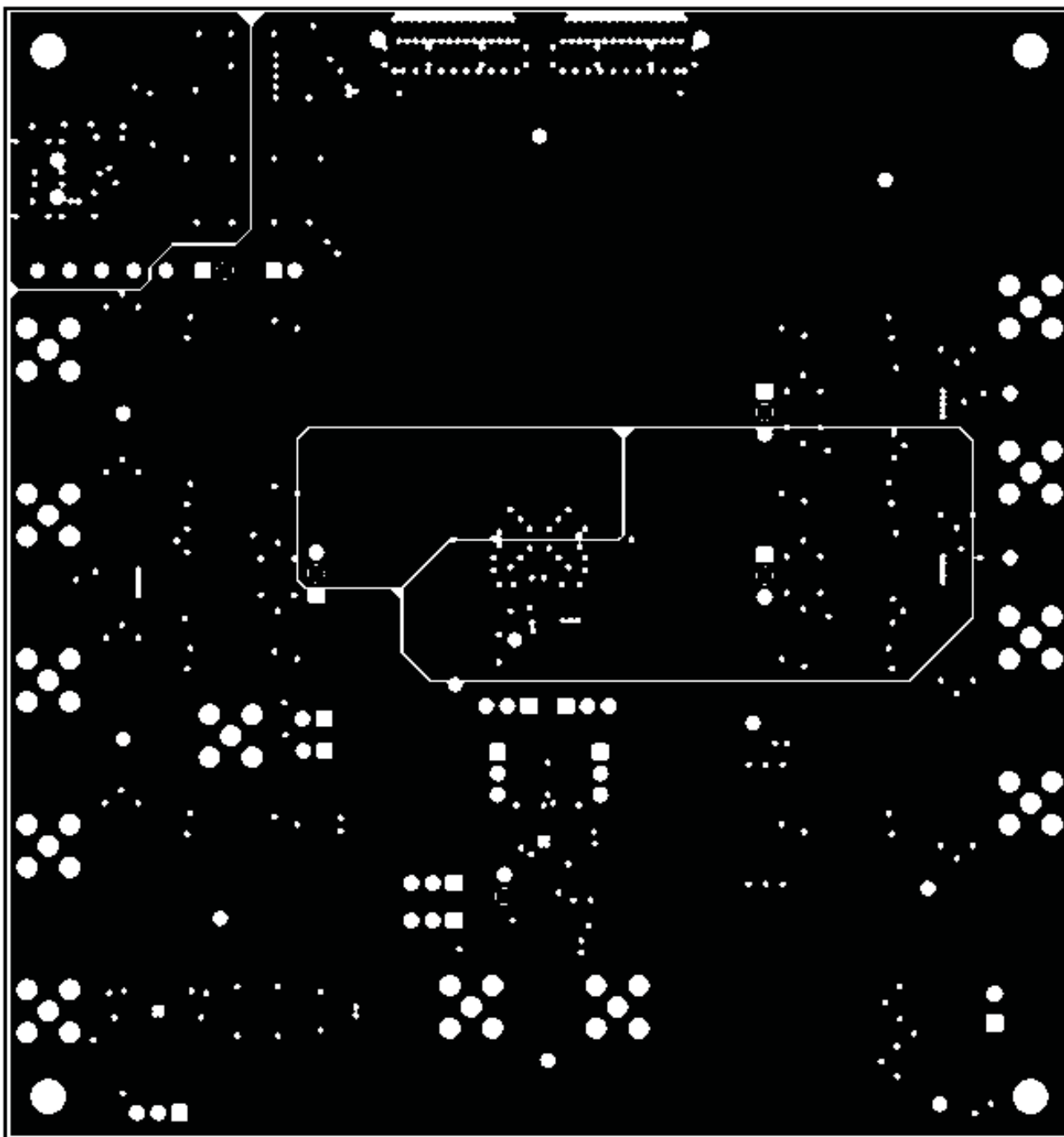
Figure 29. ADS5292EVM Internal Layer 3, Power – Top View
