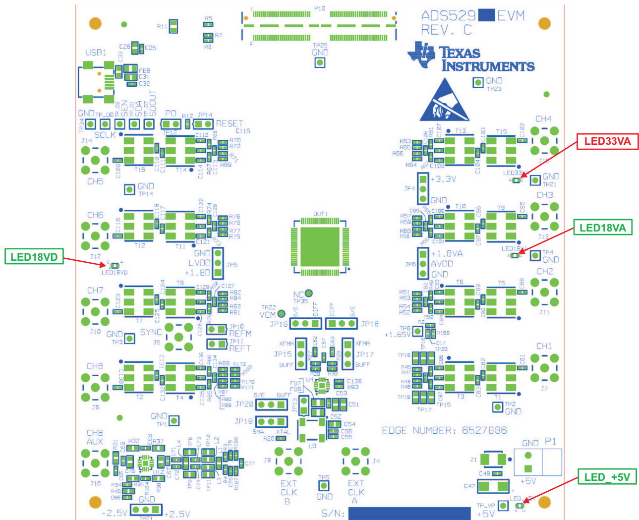
Figure 13. ADS5292EVM LED Location
