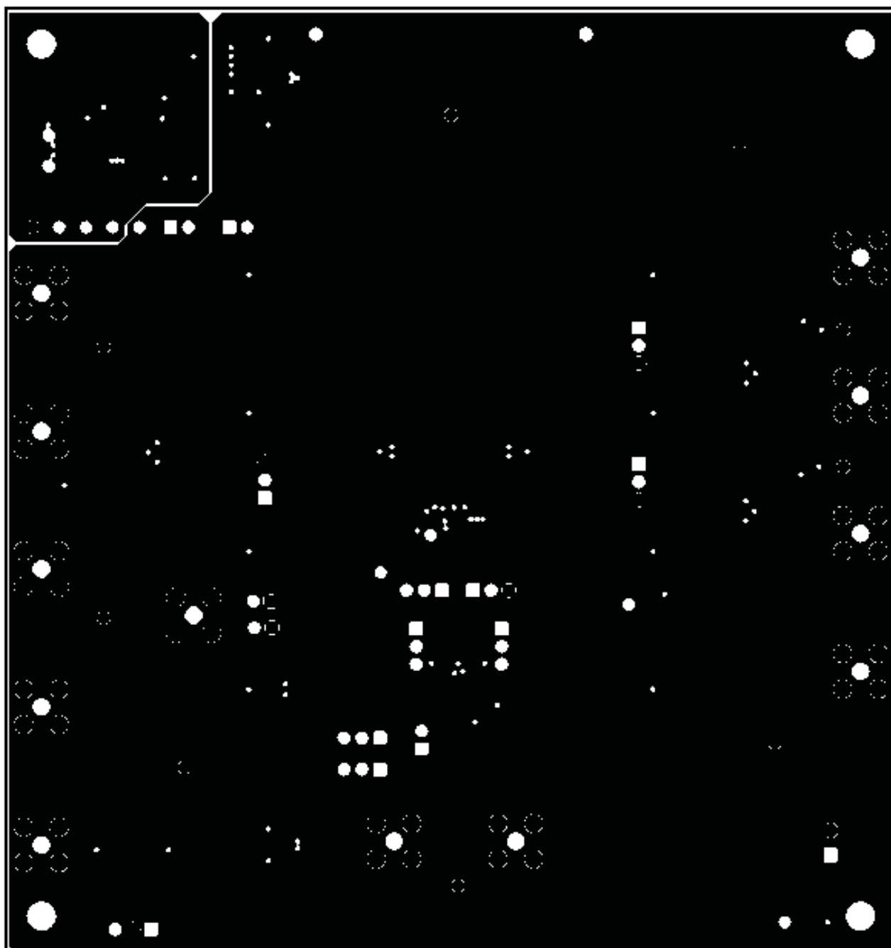
Figure 27. ADS5292EVM Internal Layer 1, Ground – Top View
