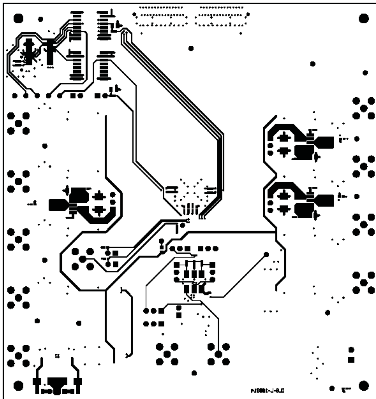
Figure 31. ADS5292EVM Bottom Layer Copper – Top View
