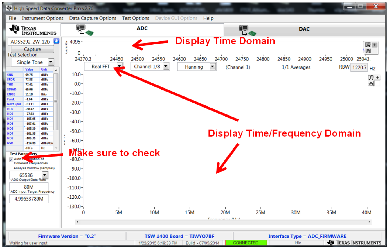
Figure 7. ADS5292 Time Domain Setup
