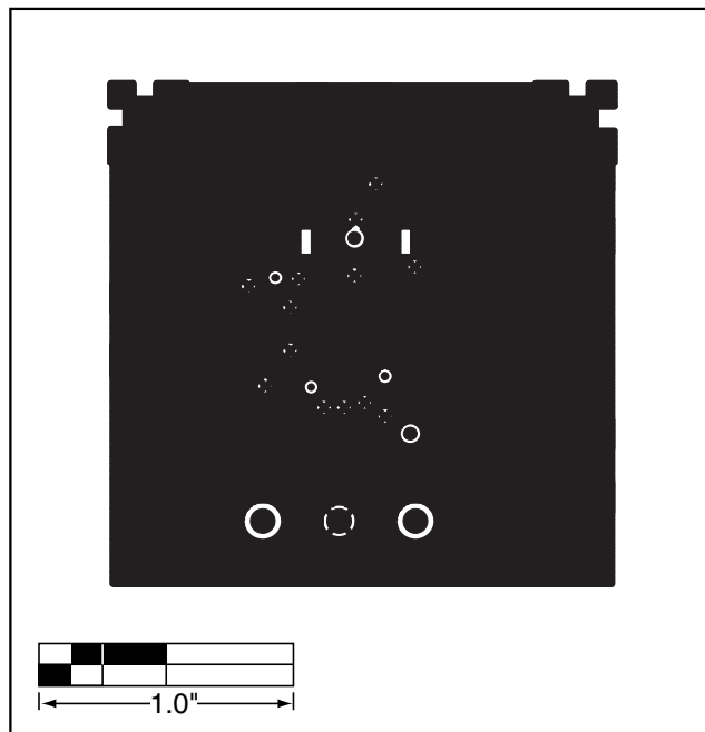
Figure 6. MAX9993 EV Kit PC Board Layout— Inner Layer 2 (GND)
