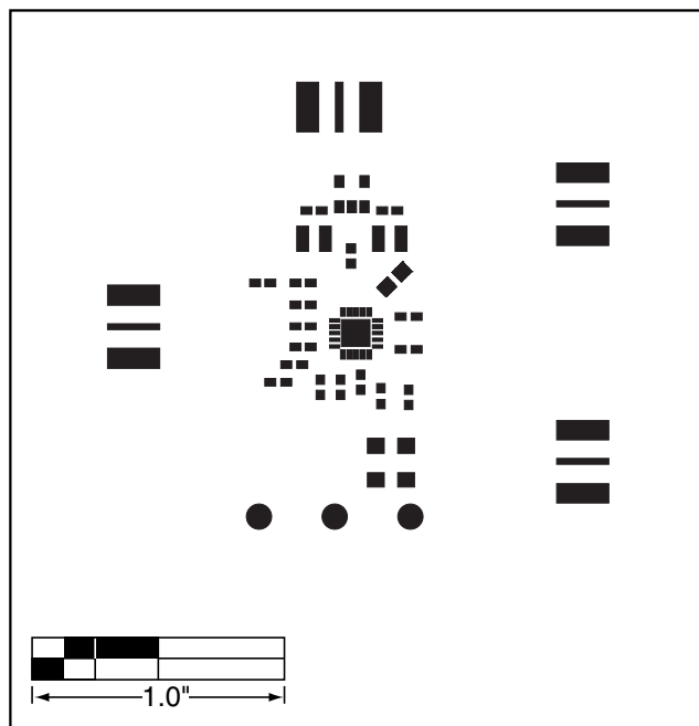
Figure 4. MAX9993 EV Kit PC Board Layout—Top Soldermask
