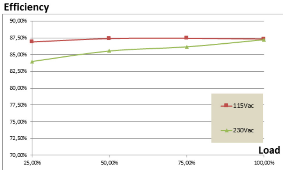
Figure 30. Board Efficiency
