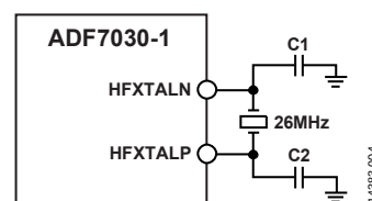
Figure 2. 26 MHz Crystal Reference Connections
