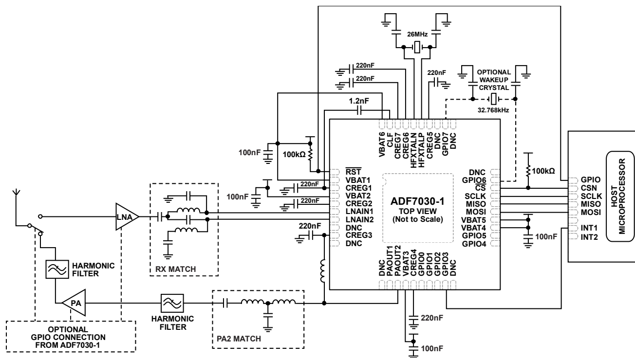
Figure 6. Application Circuit with External PA, External LNA, and a Crystal Reference
