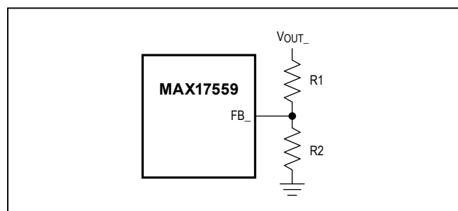
Figure 4. Output-Voltage Programming
