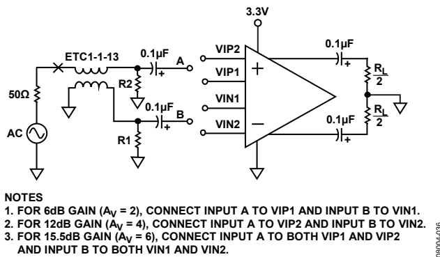
Figure 34. Differential-Input-to-Differential-Output Configuration
