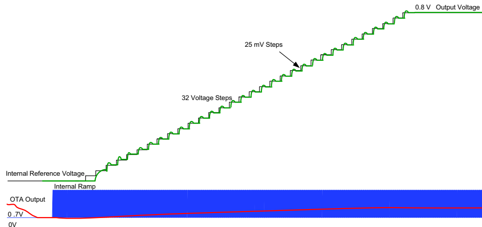
Figure 20. Soft-Start Details
