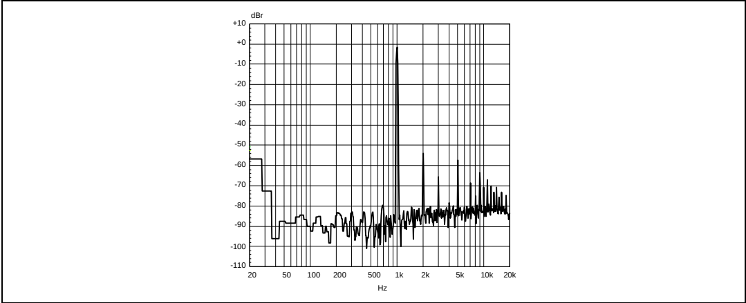
Figure 39. FFT 0 dB, 1 kHz, single ended, 4 \Omega
