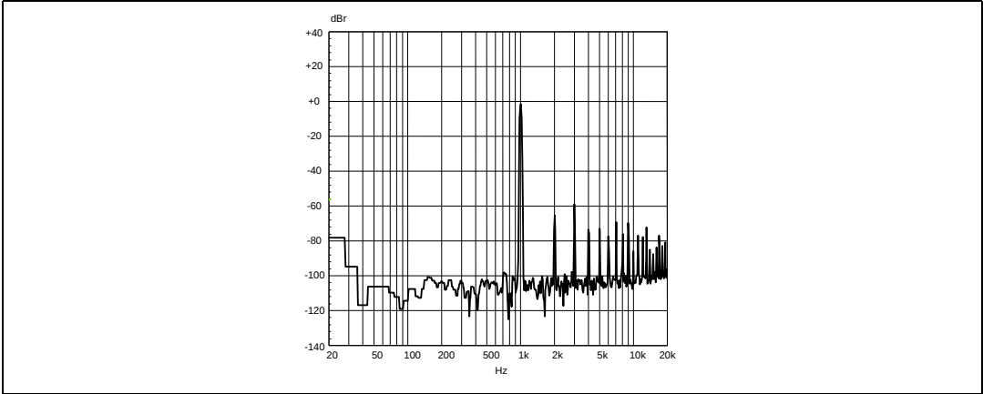
Figure 26. FFT 0 dBFS 1 kHz, 6 Ω
