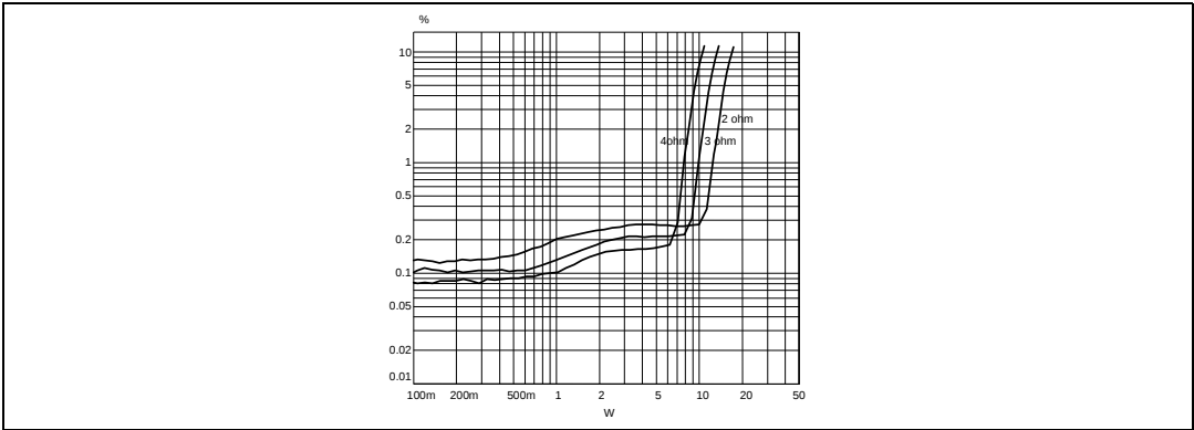
Figure 34. THD+N vs. output power, single ended, 1 kHz, half-bridge binary
