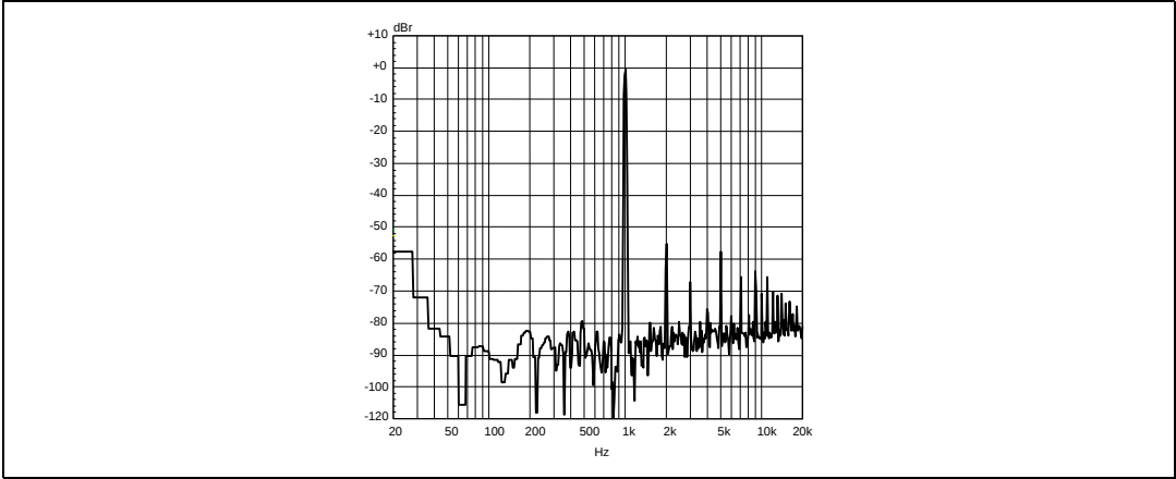
Figure 38. FFT 0 dB, 1 kHz, single ended, 3 \Omega
