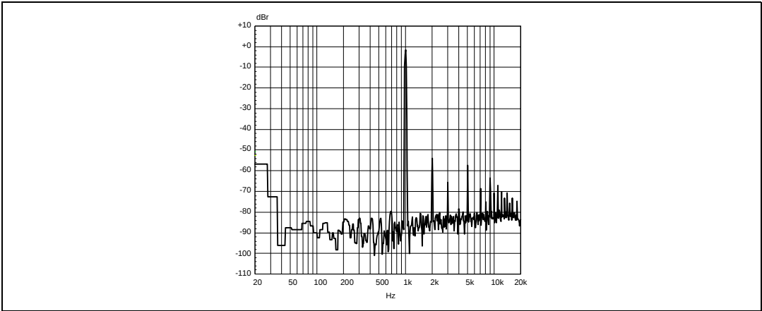
Figure 40. FFT -60 dB, single ended, 1 kHz, 2 \Omega
