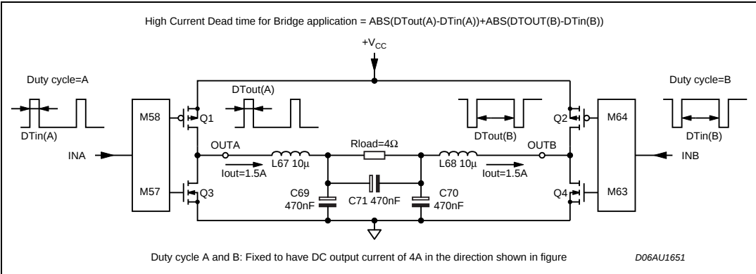
Figure 10. Test circuit 2
