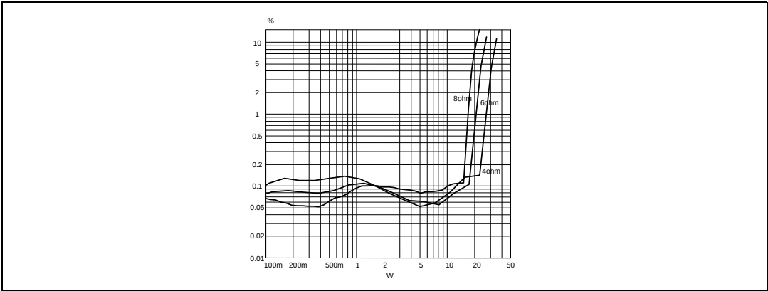
Figure 22. THD vs. output power, BTL, 1 kHz
