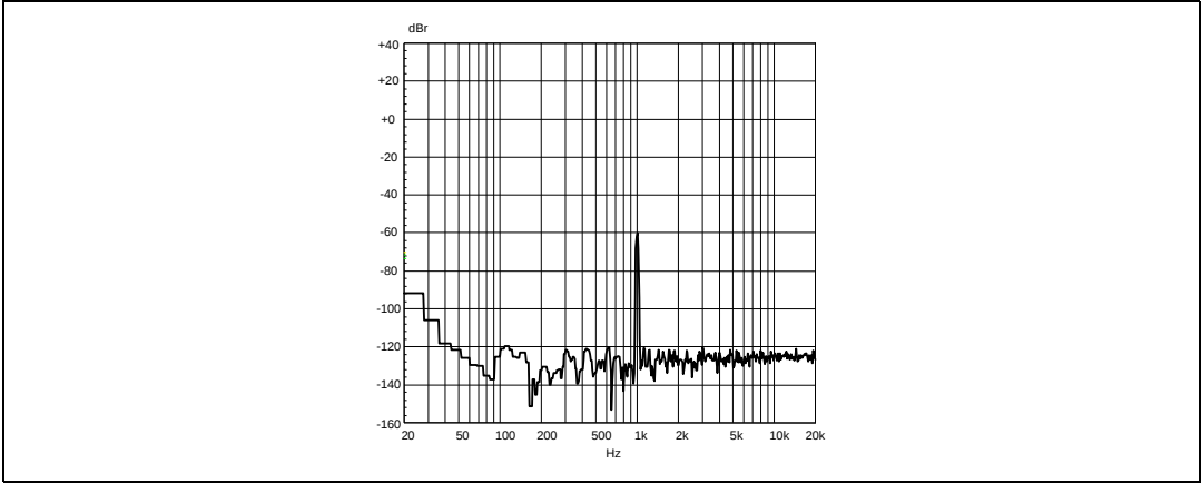
Figure 30. FFT -60 dBFS 1 kHz, 4 \Omega
