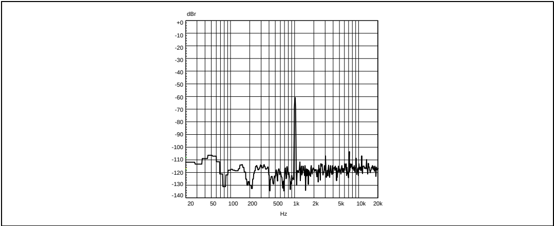
Figure 41. FFT -60 dB, single ended, 1 kHz, 4 \Omega
