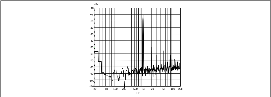
Figure 37. FFT 0 dB, 1 kHz, single ended, 2 \Omega
