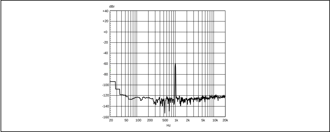
Figure 29. FFT -60 dBFS 1 kHz, 6 \Omega
