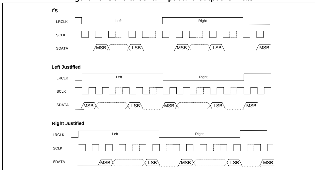
Figure 46. General serial input and output formats
