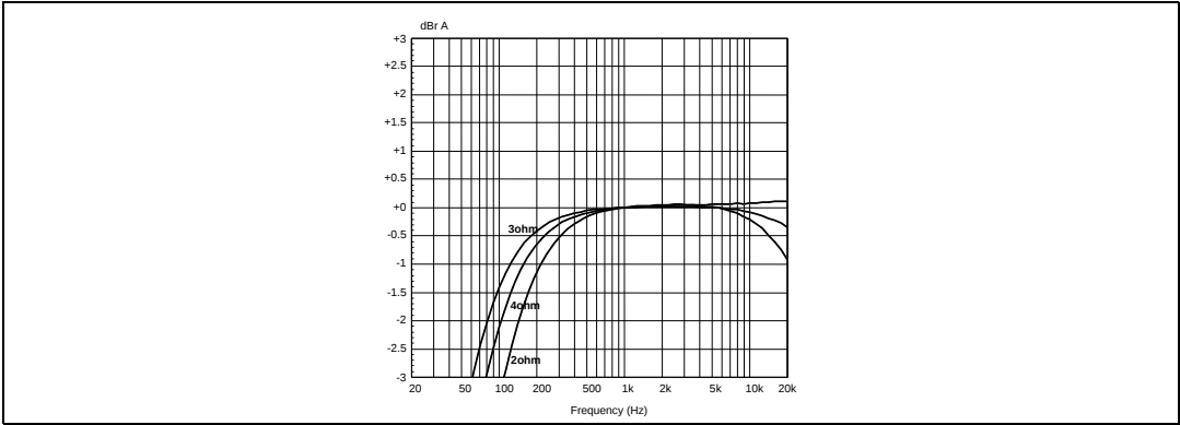
Figure 32. Frequency response, 1 W, binary half-bridge mode
