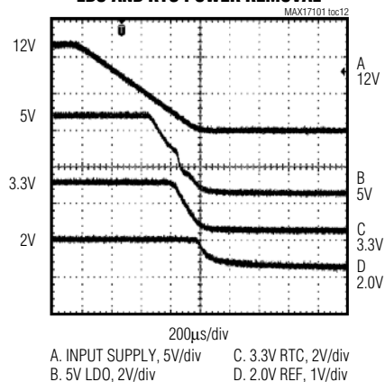
LDO AND RTC POWER REMOVAL
