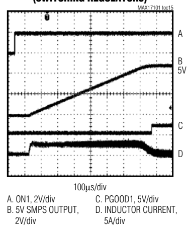
STARTUP WAVEFORMS (SWITCHING REGULATORS)
