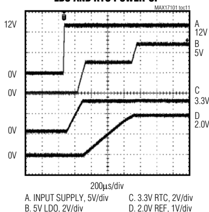
LDO AND RTC POWER-UP
