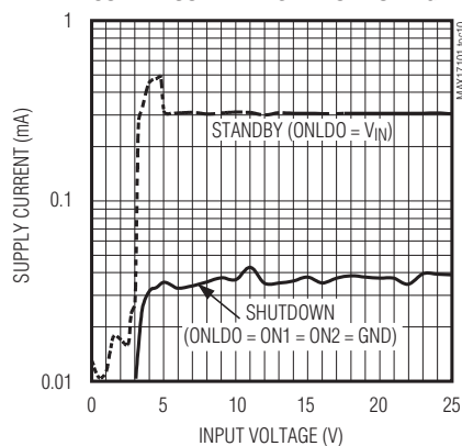
STANDBY AND SHUTDOWN INPUT SUPPLY CURRENT vs. INPUT VOLTAGE
