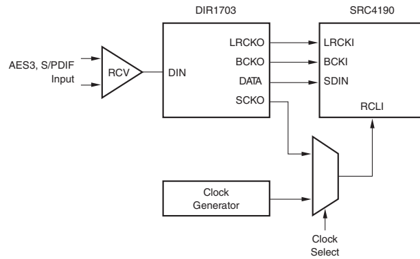
Figure 9. Interfacing the SRC4190 to the DIR1703 Digital Audio Interface Receiver
