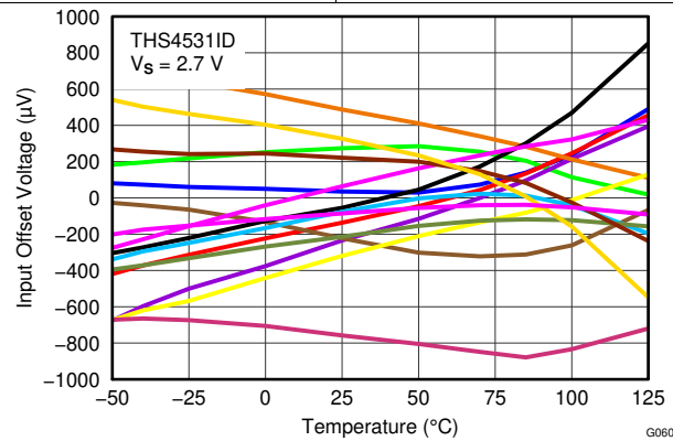
Figure 34. Input Offset Voltage vs Temperature
