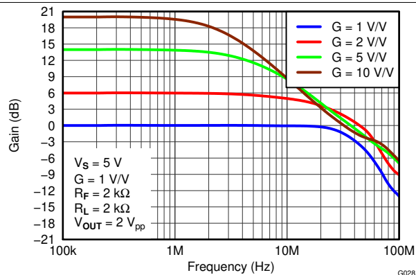
Figure 36. Large-Signal Frequency Response
