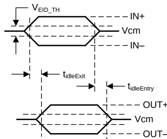
Figure 2. Electrical Idle Mode Exit and Entry Delay Timing
