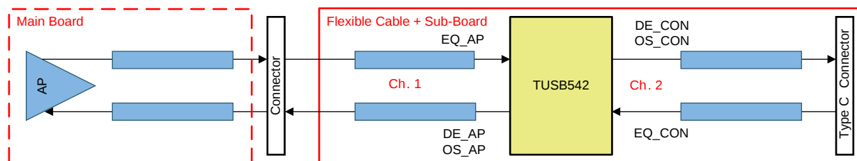
Figure 13. Typical Channels
