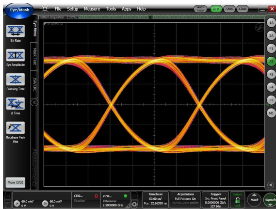
Figure 5. Output Signal: 12-Inches Output Trace
