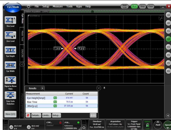
Figure 11. Output Signal: 12-Inches Output Trace
