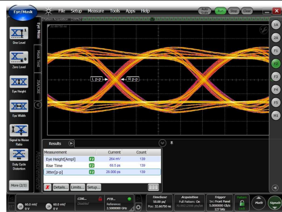
Figure 12. Output Signal: 24-Inches Output Trace
