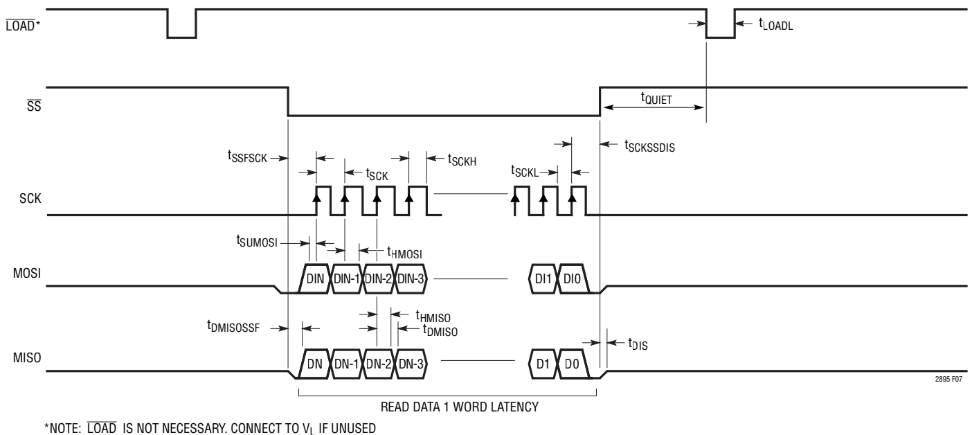
Figure 7. Logic Side Interface
