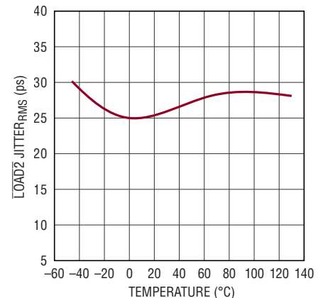
LOAD2 Jitter RMS vs Temperature
