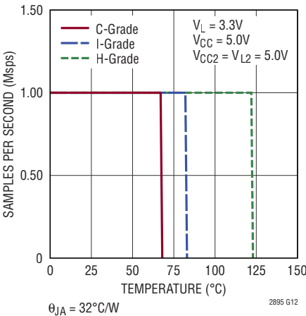
Temperature Derating Curve
