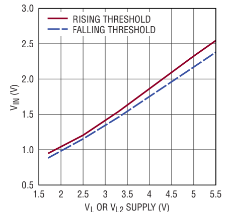
LOAD or MOSI, SCK, \overline{\text{SS}} , \overline{\text{SSB}} , MIS02 Inputs V_{IN} Thresholds vs V_L or V_{L2}
