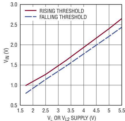
SA, SB, SC, SA2, SB2, or SC2 as Inputs V_{IN} Thresholds vs V_L or V_{L2}
