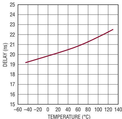
LOAD to LOAD2 Delay vs Temperature
