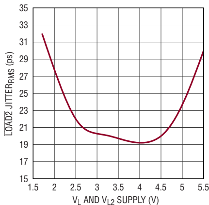
LOAD2 Jitter RMS vs V_L and V_{L2}
