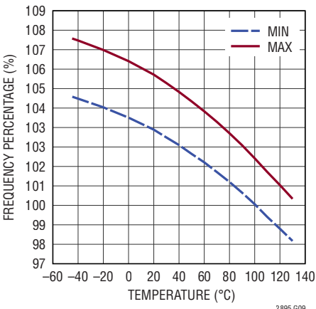
SCK2 Frequency Variation vs Temperature
