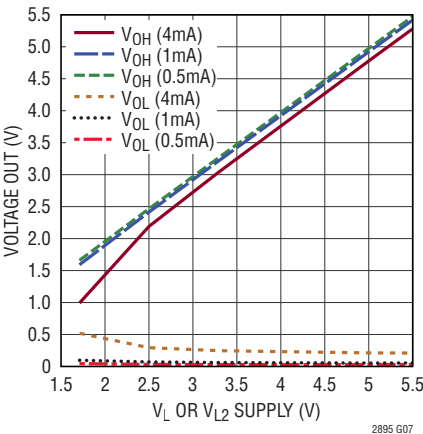
SA, SB, SC, SA2, SB2, or SC2 as Outputs V_{OL}/V_{OH} vs V_L or V_{L2} Voltage
