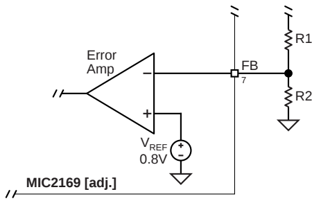
Figure 2. Voltage-Divider Configuration
