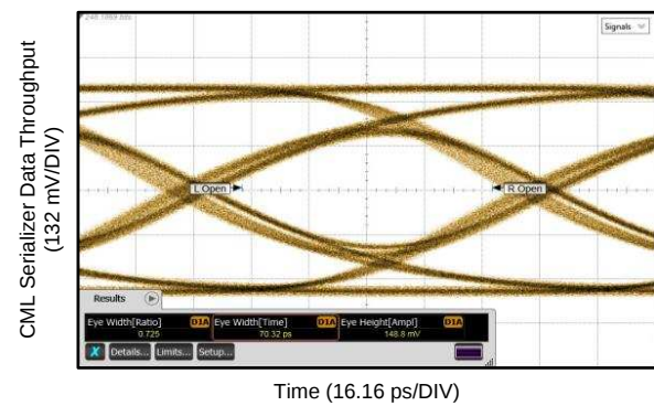
Figure 32. TL1 = 15 Inch 4-Mil FR4 Trace, TL2 = 10 Inch 4-Mil FR4 Trace, DS100BR210 CHA, 10.3125 Gbps
