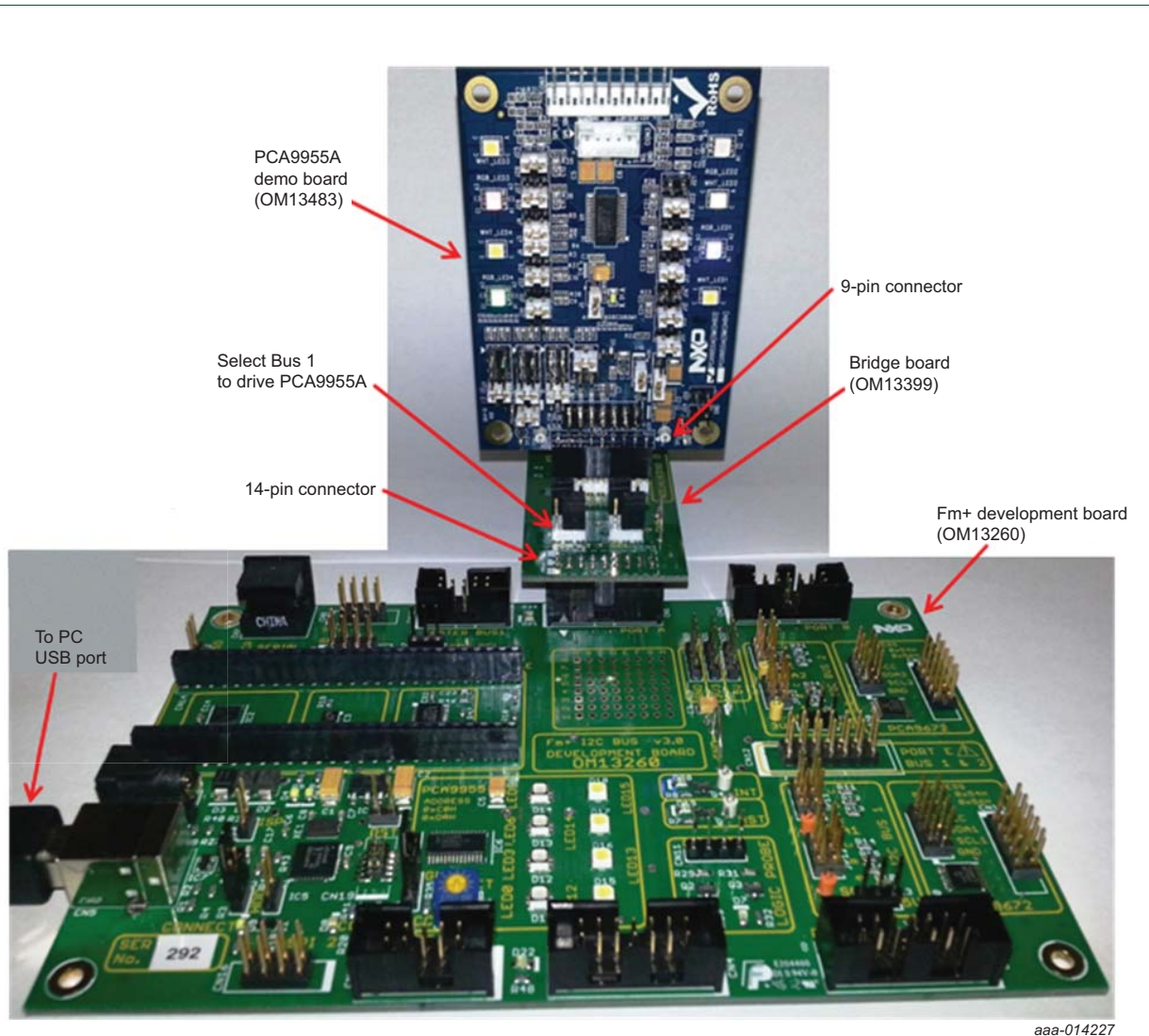
Fig 2. PCA9955A/B demo board (OM13483) mounting to the Fm+ development board (OM13260)
