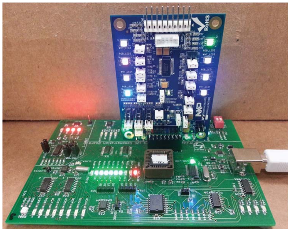
Fig 1. PCA9955A/B demo board (OM13483) mounting to the I2C demo board 2005-1 (OM6275)
