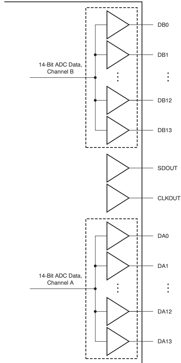
Figure 47. CMOS Outputs
