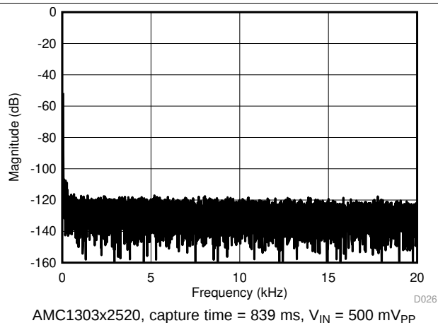
Figure 34. Frequency Spectrum With 35-Hz Input Signal
