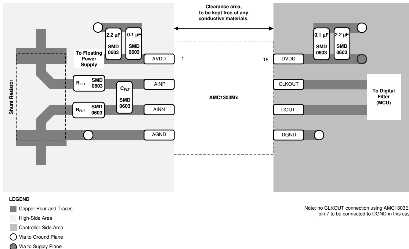
Figure 58. Recommended Layout of the AMC1303
