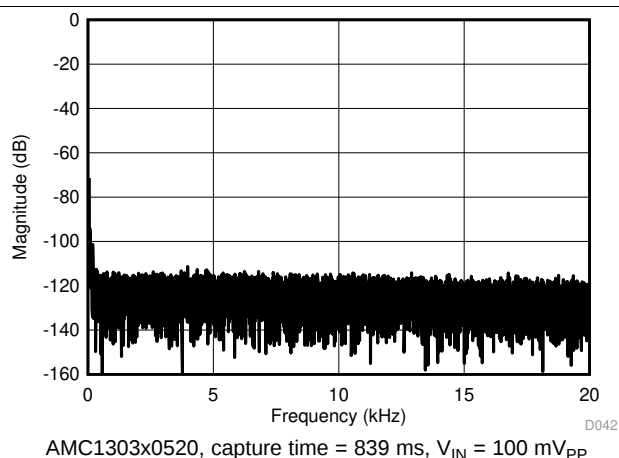
Figure 32. Frequency Spectrum With 35-Hz Input Signal
