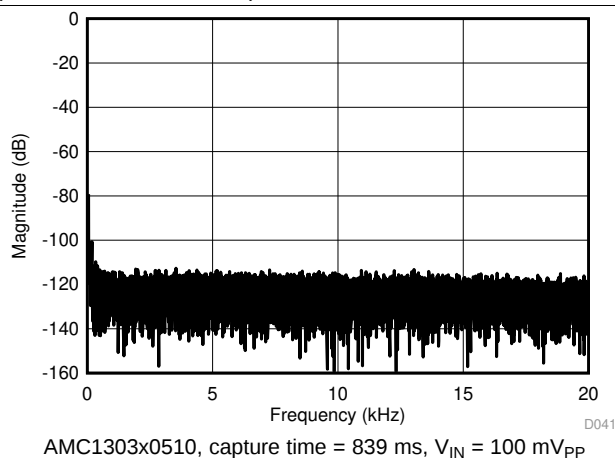
Figure 31. Frequency Spectrum With 35-Hz Input Signal
