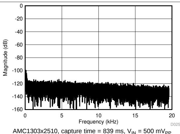
Figure 33. Frequency Spectrum With 35-Hz Input Signal
