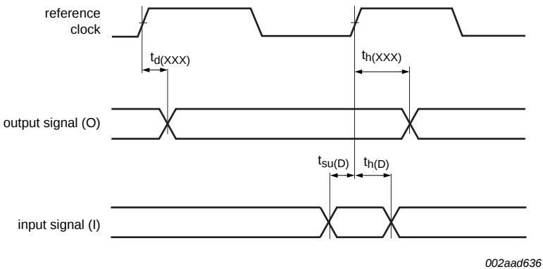
Fig 18. Signal timing
