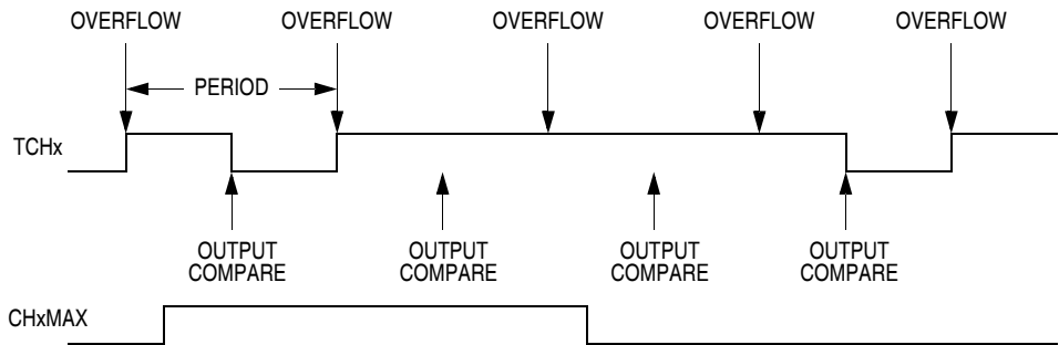
Figure 18-12. CHxMAX Latency
