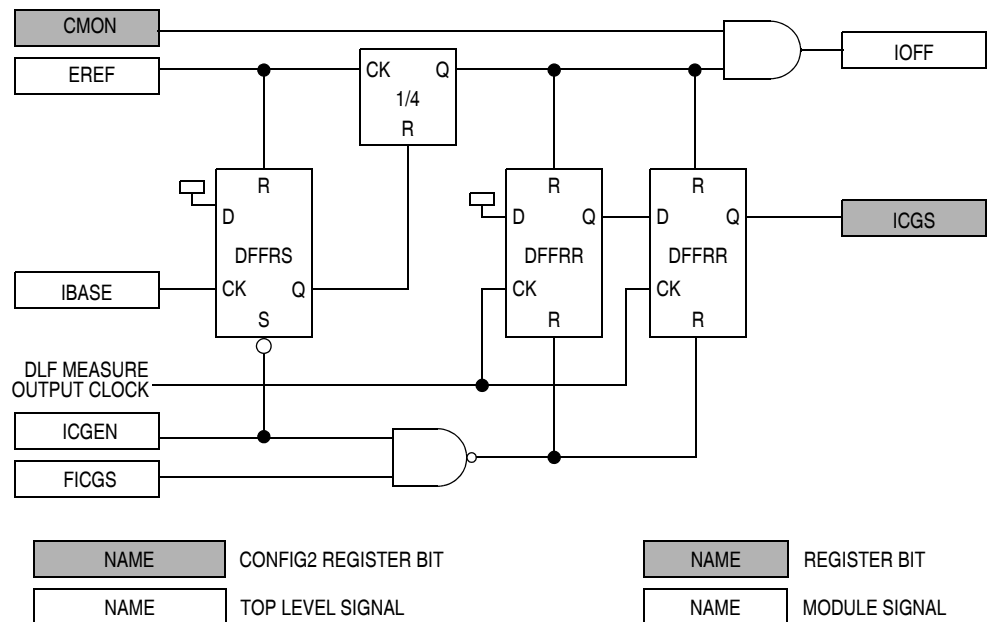
Figure 7-6. Internal Clock Activity Detector
