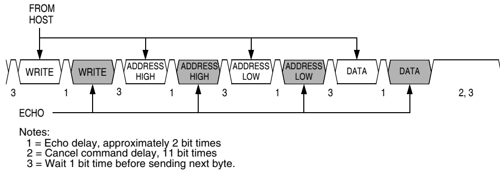
Figure 19-16. Write Transaction
