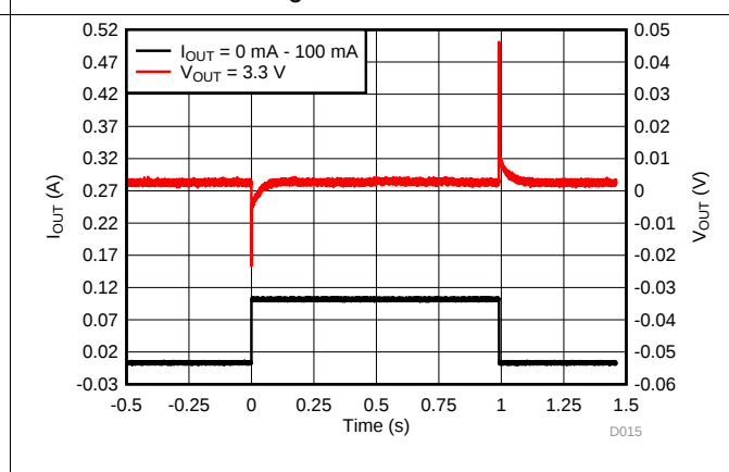
Figure 16. Load Transient
