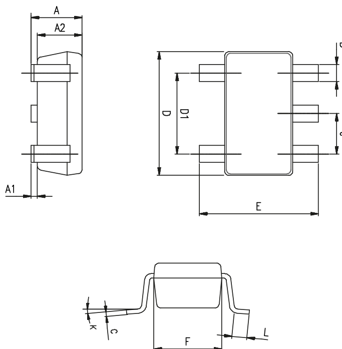
Figure 47. SOT23-5 package outline
