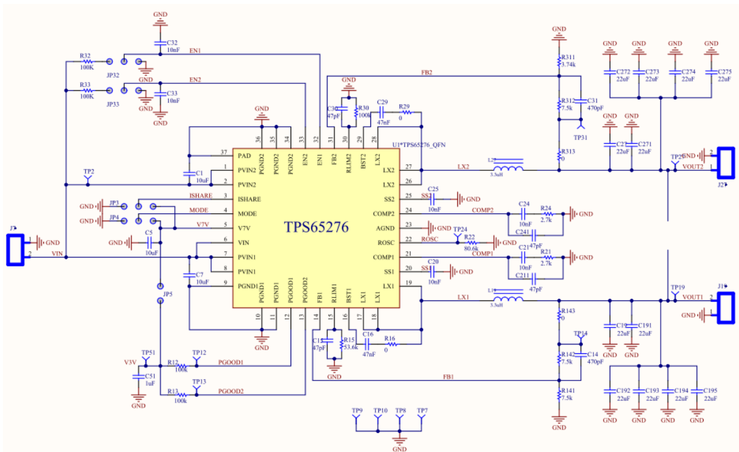
Figure 1. TPS65276 Schematic
