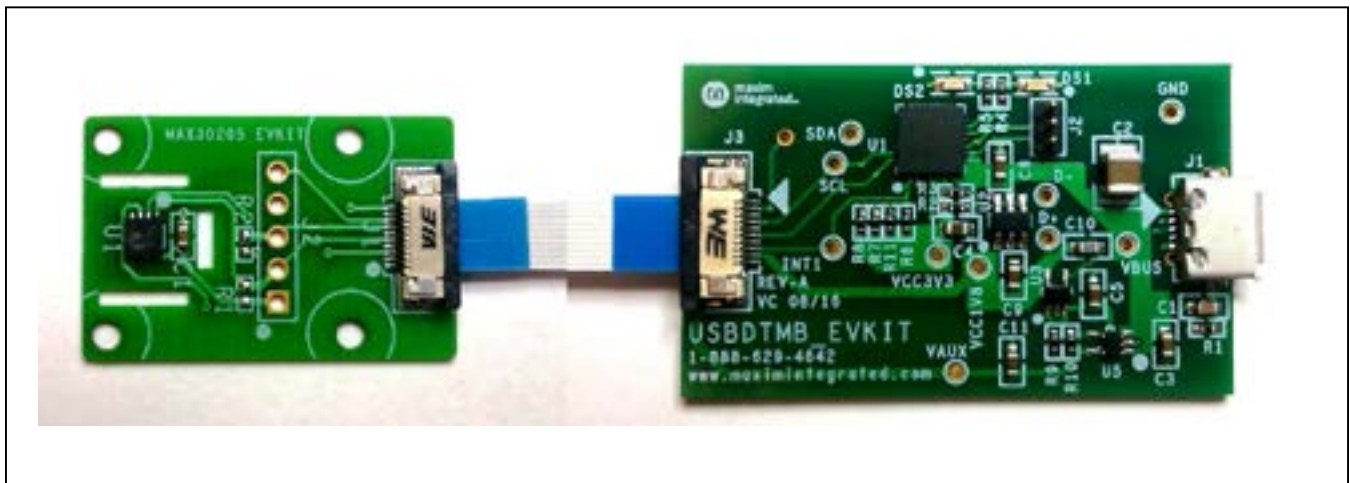
Figure 1. MAX30205 EV Kit Temperature Sensor and USBDTMB Controller PCB
