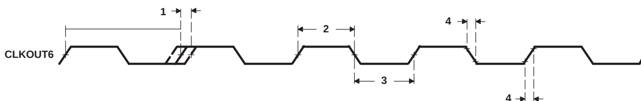
Figure 5-7. CLKOUT6 Timing
