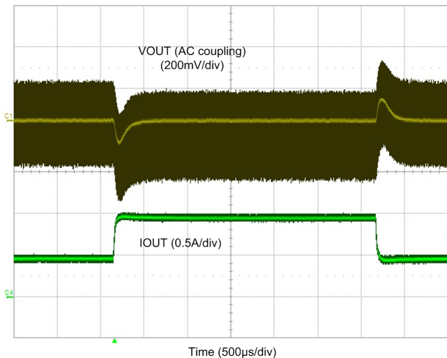
Figure 4. Load Transient Response (VIN = 36 V)
