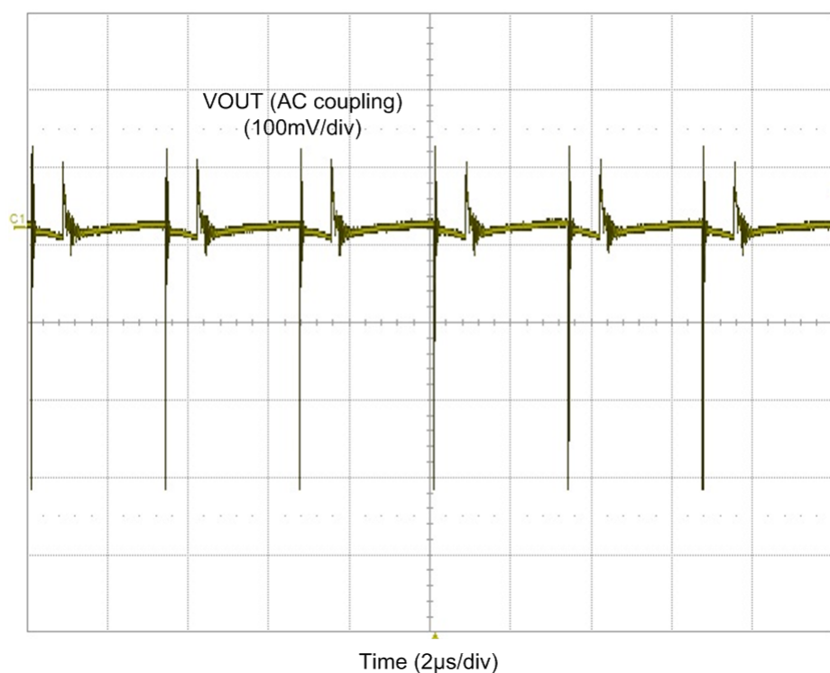
Figure 3. Output Voltage Ripple (VIN = 36 V, IOUT = 2 A)
