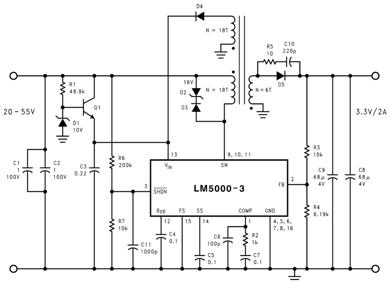
Figure 5. Non-Isolated Flyback Converter Schematic
