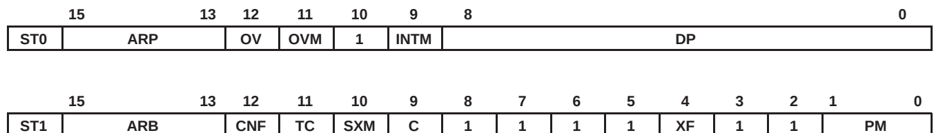
Figure 13. Organization of Status Registers ST0 and ST1
