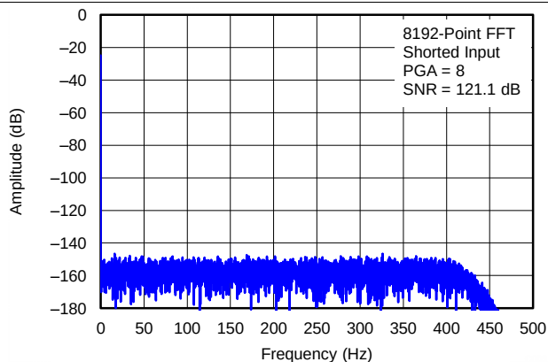
Figure 2. Output Spectrum
