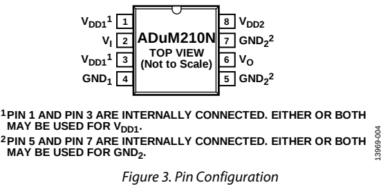
Figure 3. Pin Configuration
