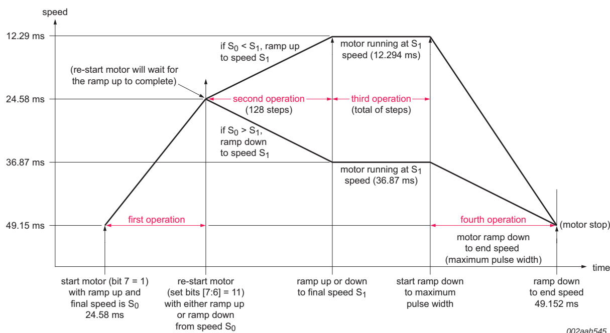
Fig 15. Re-start motor with ramp-up/ramp-down enable while current motor running in the ramp-up
