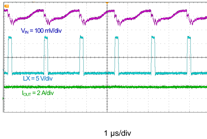
Figure 8. TPS564208 Input Voltage Ripple
