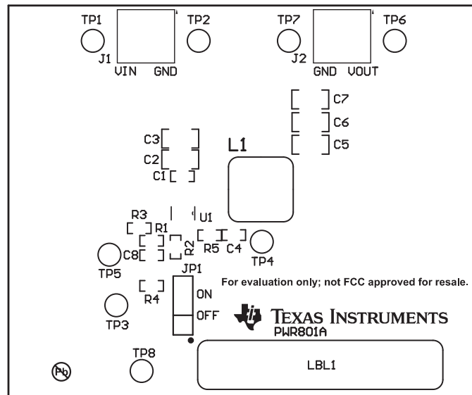
Figure 13. Top Assembly
