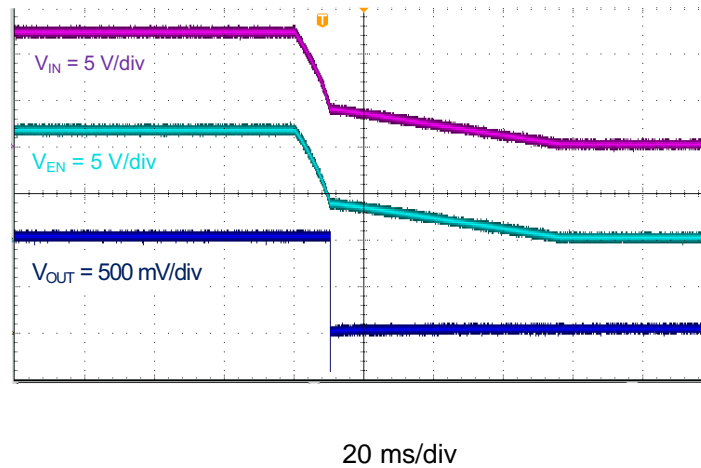
Figure 11. TPS564208 Shut-Down Relative to V_{IN}
