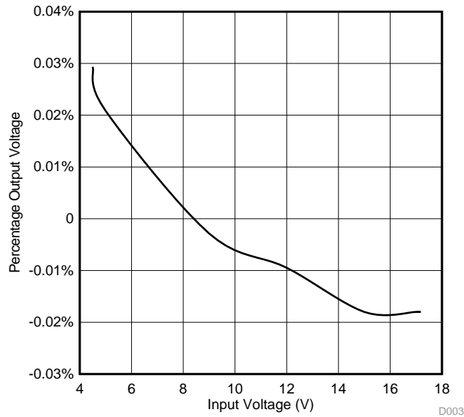
Figure 3. Line Regulation
