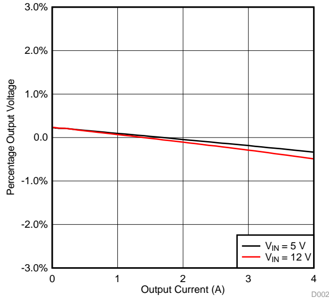
Figure 2. Load Regulation
