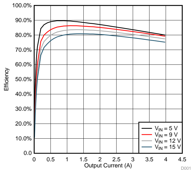
Figure 1. Efficiency
