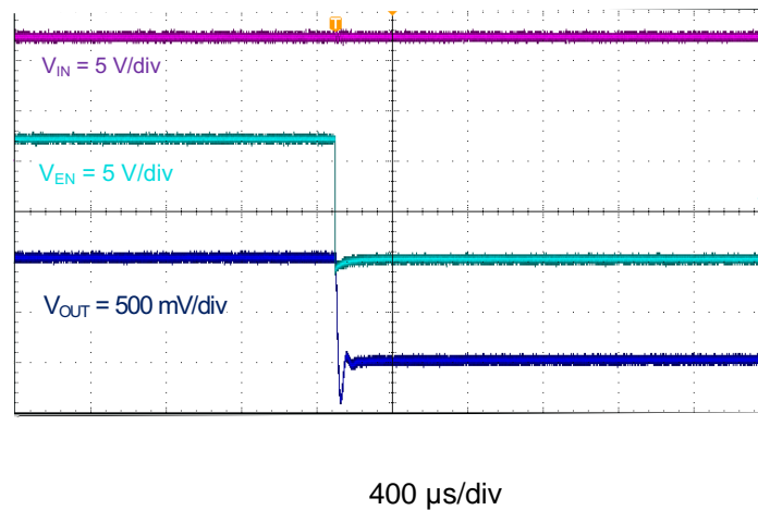
Figure 12. TPS564208 Shut-Down Relative to EN
