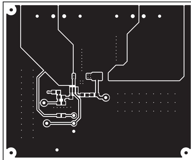
Figure 14. Top Layer
