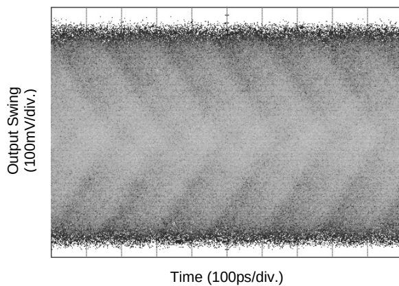
1m FR4 Output without SY58627L (6.4Gbps PRBS 2^{23} )
