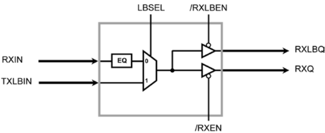
Figure 3. Loopback Control
