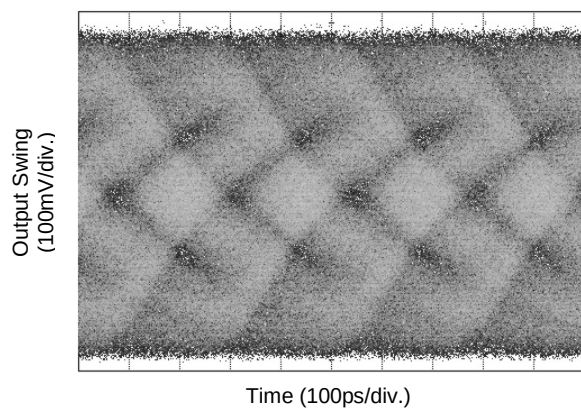
1m FR4 Output without SY58627L (4.25Gbps PRBS 2^{23} )
