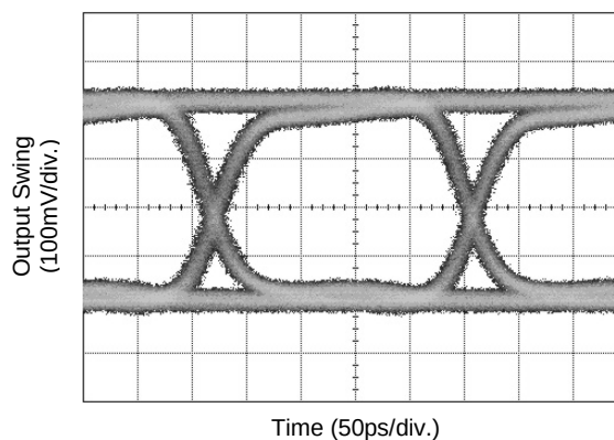
1m FR4 Output with SY58627L (4.25Gbps PRBS 2^{23} )
