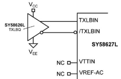
Figure 6f. TXLBIN Interface (AC-Coupled)
