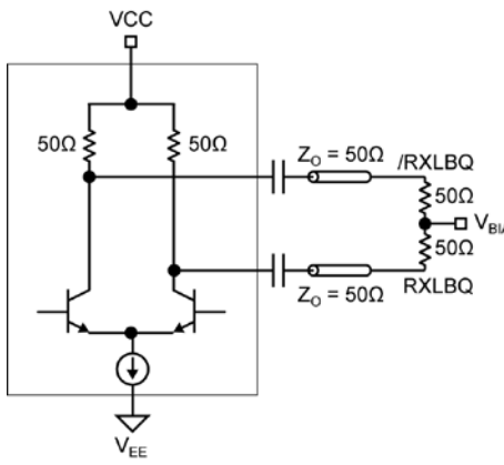
Figure 7c. CML AC-Coupled Termination
