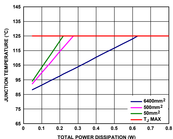
Figure 57. SOIC, T_A = 85^{\circ}\text{C}
