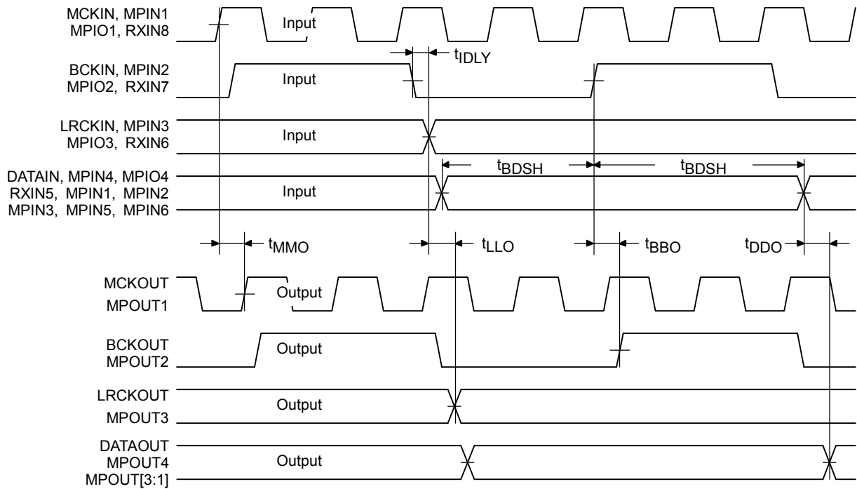
Figure 7.2 AC Characteristics 2
