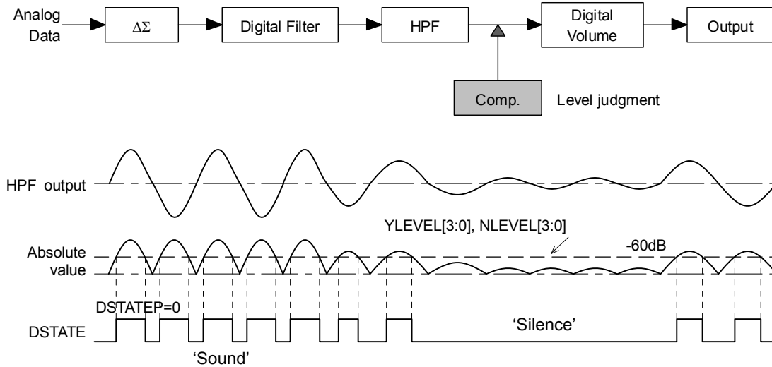
Figure 9.4 Analog Audio Data Detection Timing
