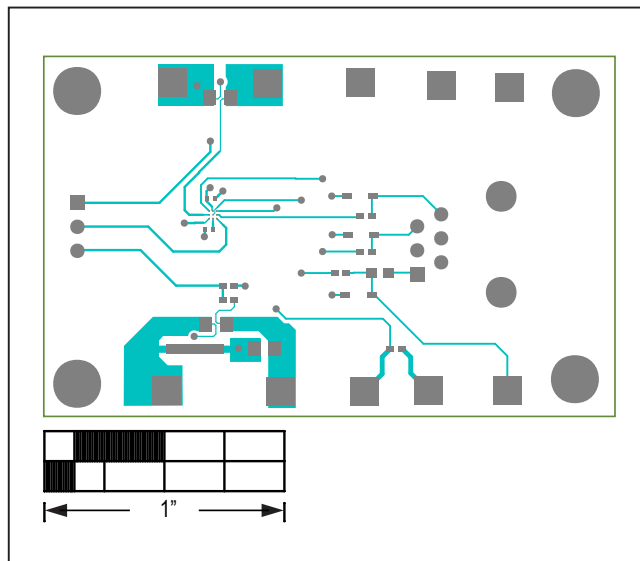
MAX17260X EV Kit PCB Layout—Top Layer
