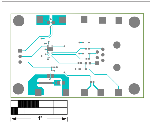
MAX17260G EV Kit PCB Layout—Top Layer
