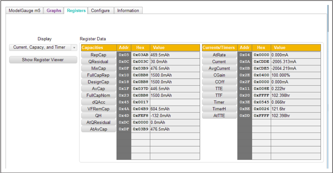
Figure 6. Registers Tab
