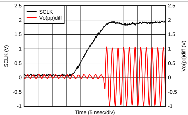
Figure 40. Gain Switching Response ( A_V = 10\text{ dB to }26\text{ dB} )
