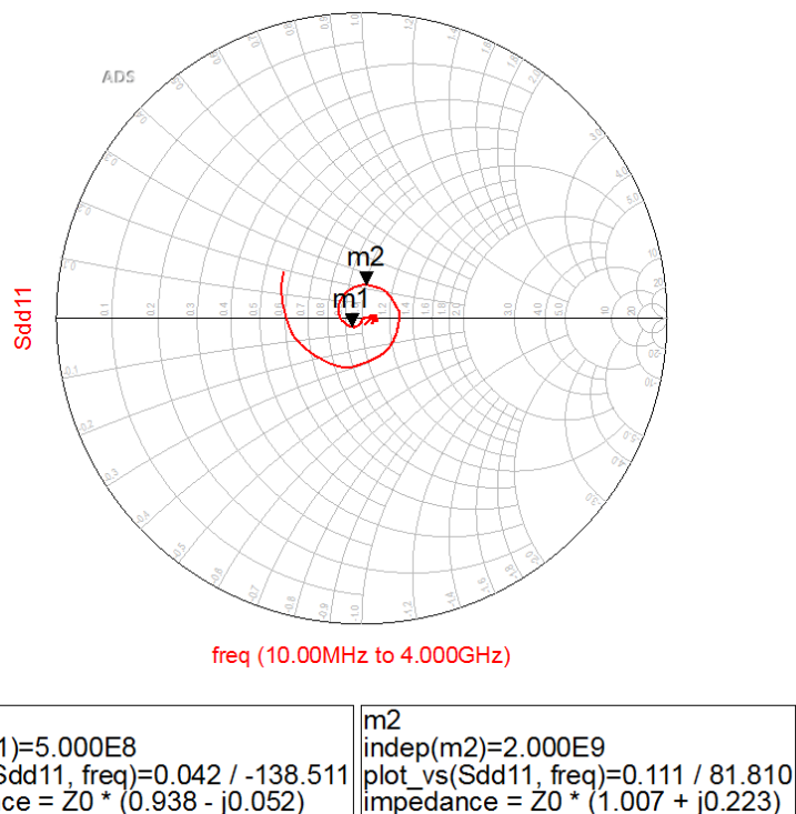
Figure 59. Smith Chart Showing Differential Input Impedance ( z_0 = 100 \Omega )
