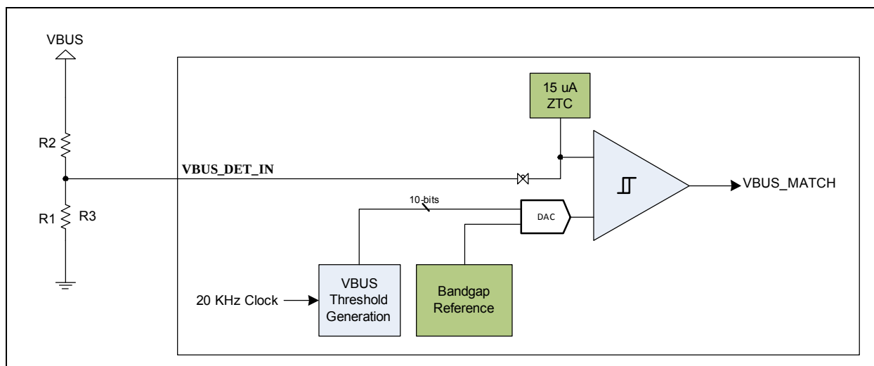
FIGURE 4-2: VBUS_DET_IN COMPARATOR
