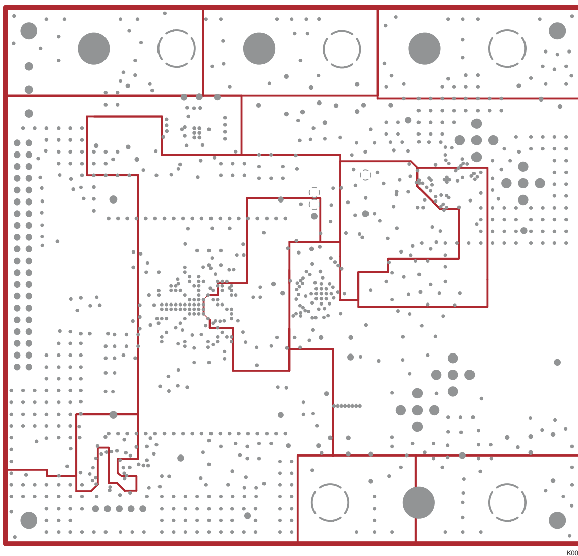
Figure 6. Layer 3, Power Plane #1
