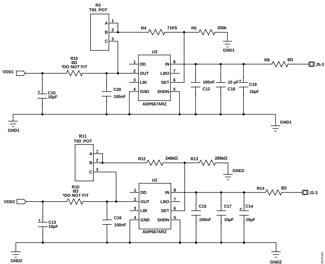
Figure 7. Schematics of the EVAL-ADM2795EEPBZ Evaluation Board, Page 2
