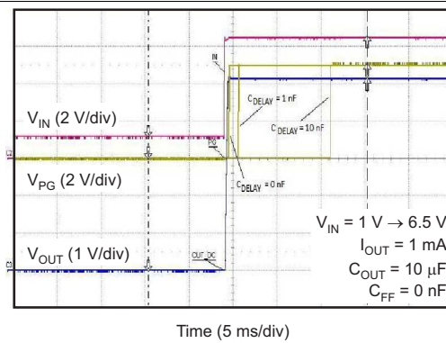
Figure 13. Power-Good Delay
