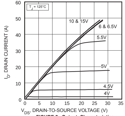
FIGURE 2, Output Characteristics
