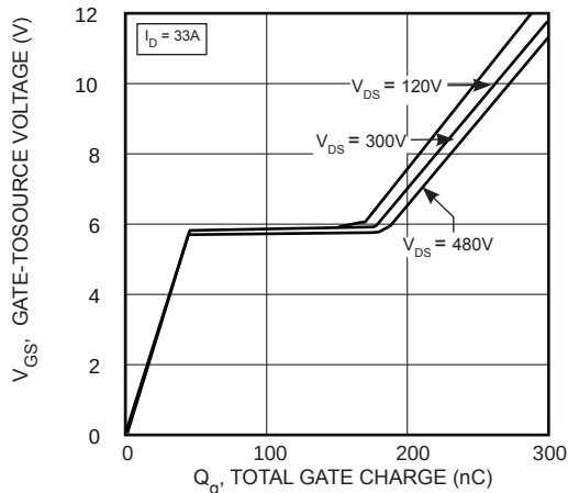
FIGURE 7, Gate Charge vs Gate-to-Source Voltage
