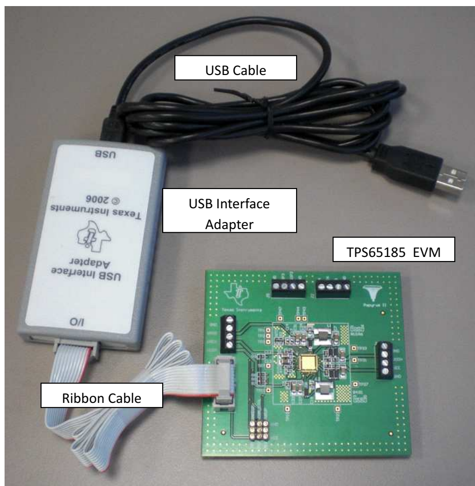
Figure 1. Included Hardware
