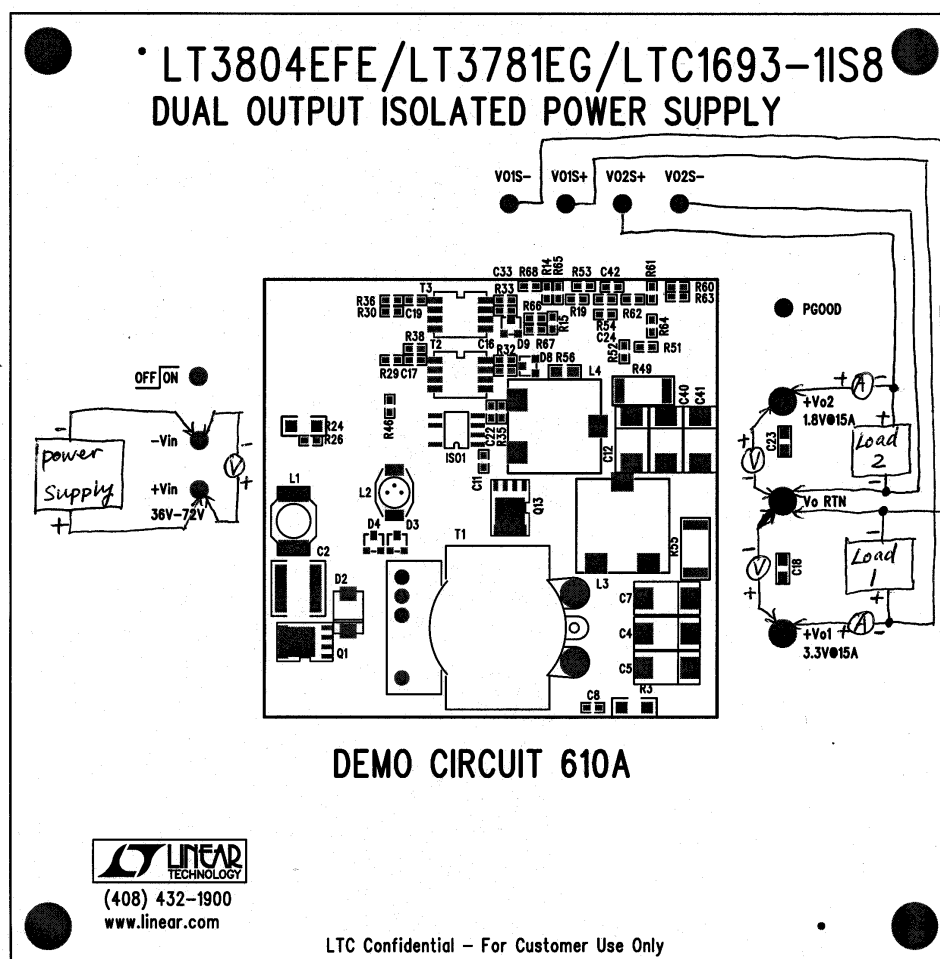
Figure 1. Proper Measurement Equipment Setup
