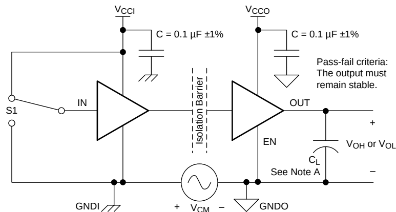
Figure 10. Common-Mode Transient Immunity Test Circuit
