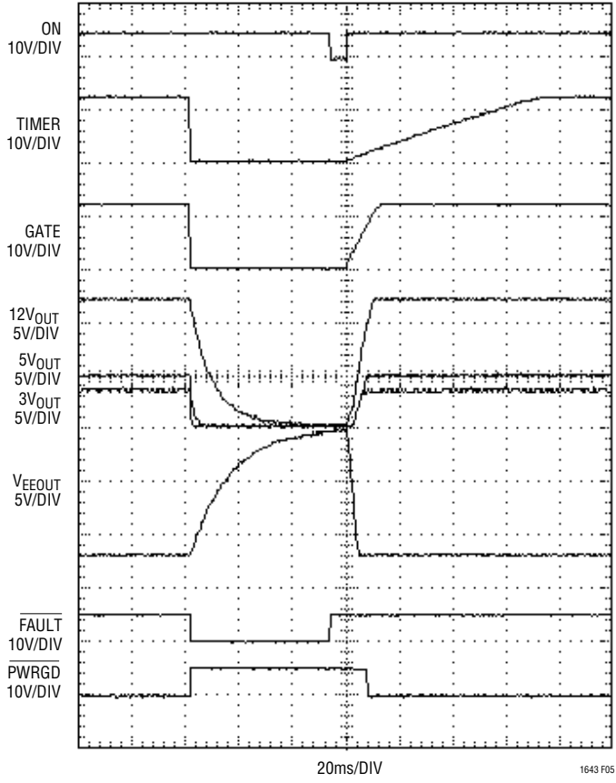
Figure 5. Short Circuit on 5V Followed by Circuit Breaker Reset
