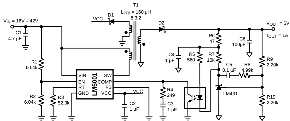
Figure 19. Isolated Flyback
