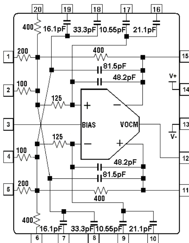
Figure 2. The LTC6601-X Circuit as configured in a DC1251A assembly.
