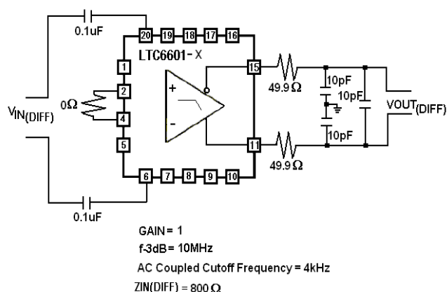
Figure 2. The LTC6601-X Circuit as configured in a DC1251A assembly.
