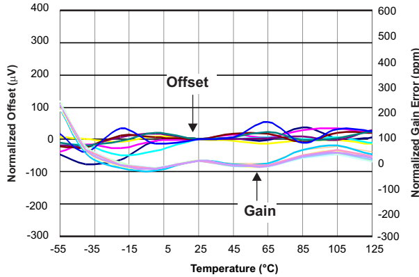
OFFSET AND GAIN vs TEMPERATURE
