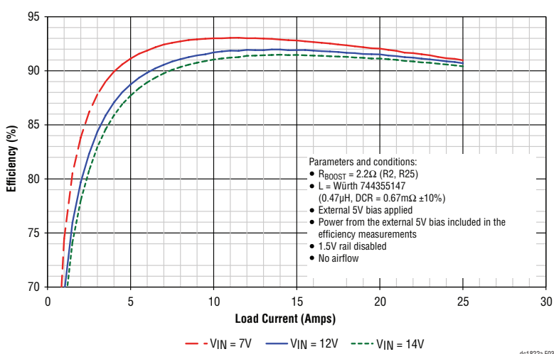
Figure 3. Efficiency Curves for the 1.2V Rail of the DC1822A. f_{\text{SW}} = 500\text{kHz} with the FDMF6820A DrMOS
