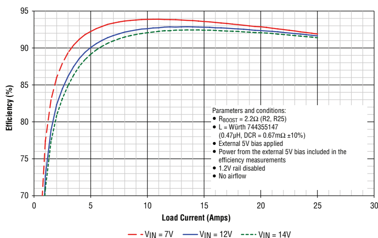
Figure 2. Efficiency Curves for the 1.5V Rail of the DC1822A. f_{\text{SW}} = 500\text{kHz} with the FDMF6820A DrMOS
