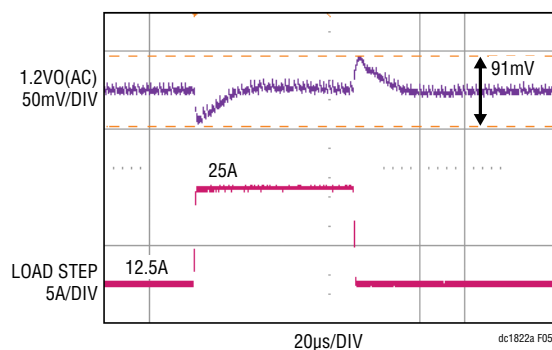
Figure 5. Load Step Response of the DC1822A 1.2V Rail at V_{IN} = 12V . C_{OUT} = 3 \times \text{Sanyo 2R5TPE330M9} \parallel 2 \times 100\mu F \text{ X5R 6.3V 1210} , L = 0.47\mu H , f_{SW} = 500kHz
