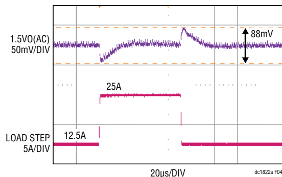
Figure 4. Load Step Response of the DC1822A 1.5V Rail at V_{IN} = 12V . C_{OUT} = 3 \times \text{Sanyo 2R5TPE330M9} \parallel 2 \times 100\mu F \text{ X5R 6.3V 1210} , L = 0.47\mu H , f_{SW} = 500kHz
