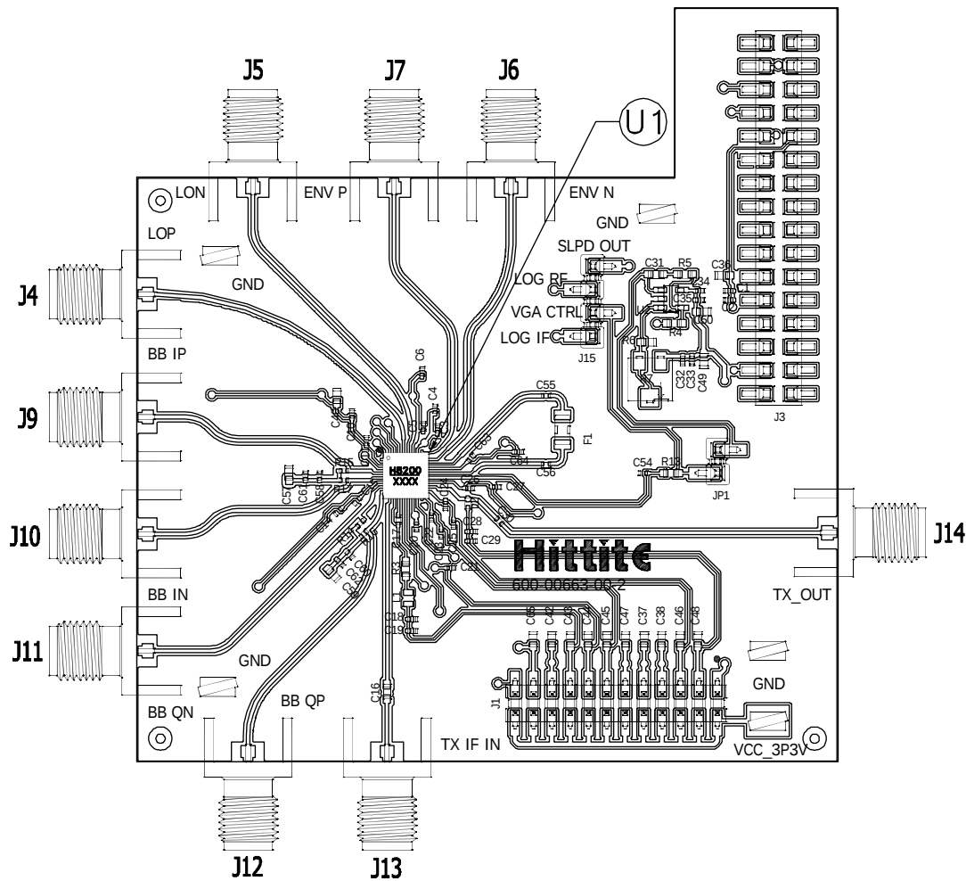
Figure 63. Evaluation PCB
